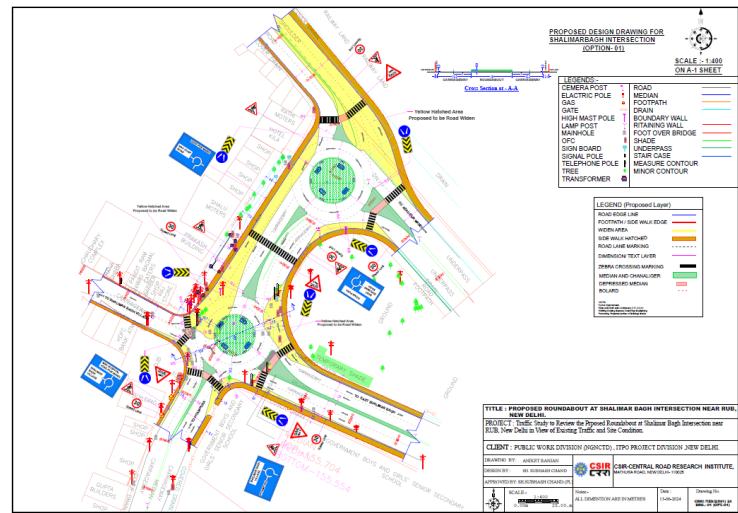
Figure 4: Geometric Layout Design of the recommended Design
