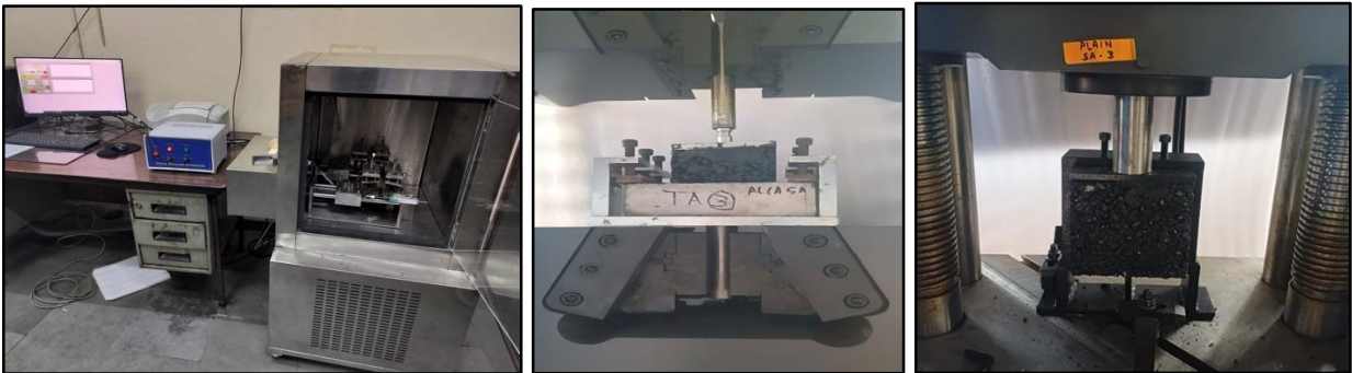
Figure 1: Development of Test Set Up for (a) Crack Bridging Test (b) Tensile Strength Test (c) Shear Adhesion Test
