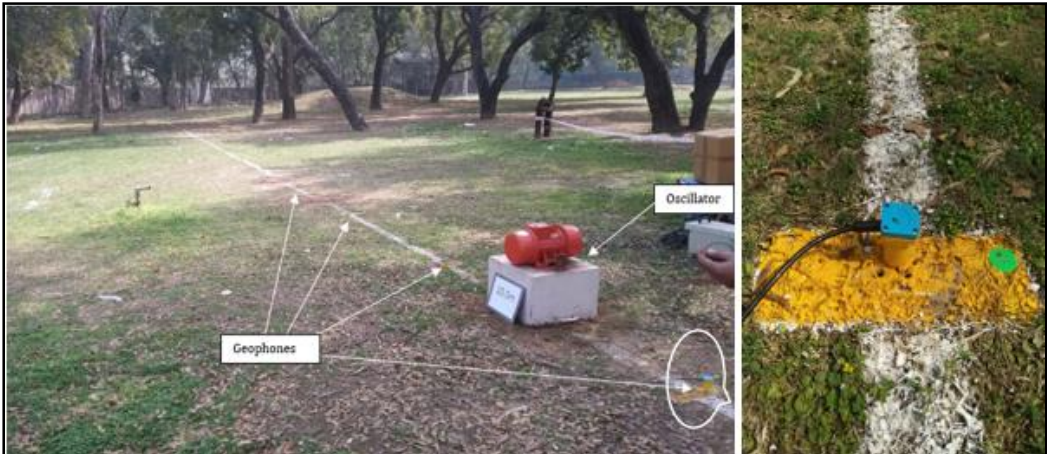
Figure 10: Instrumentation Setup showing Placement of Oscillator and Installed Geophones
