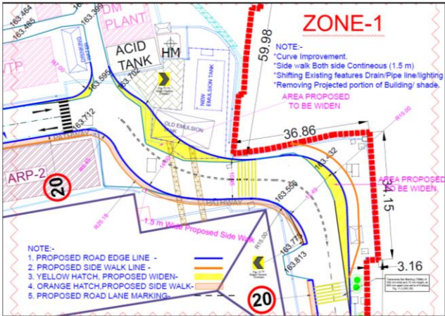
Figure 6: Proposed Infrastructure Improvement Proposal at Zone-1
