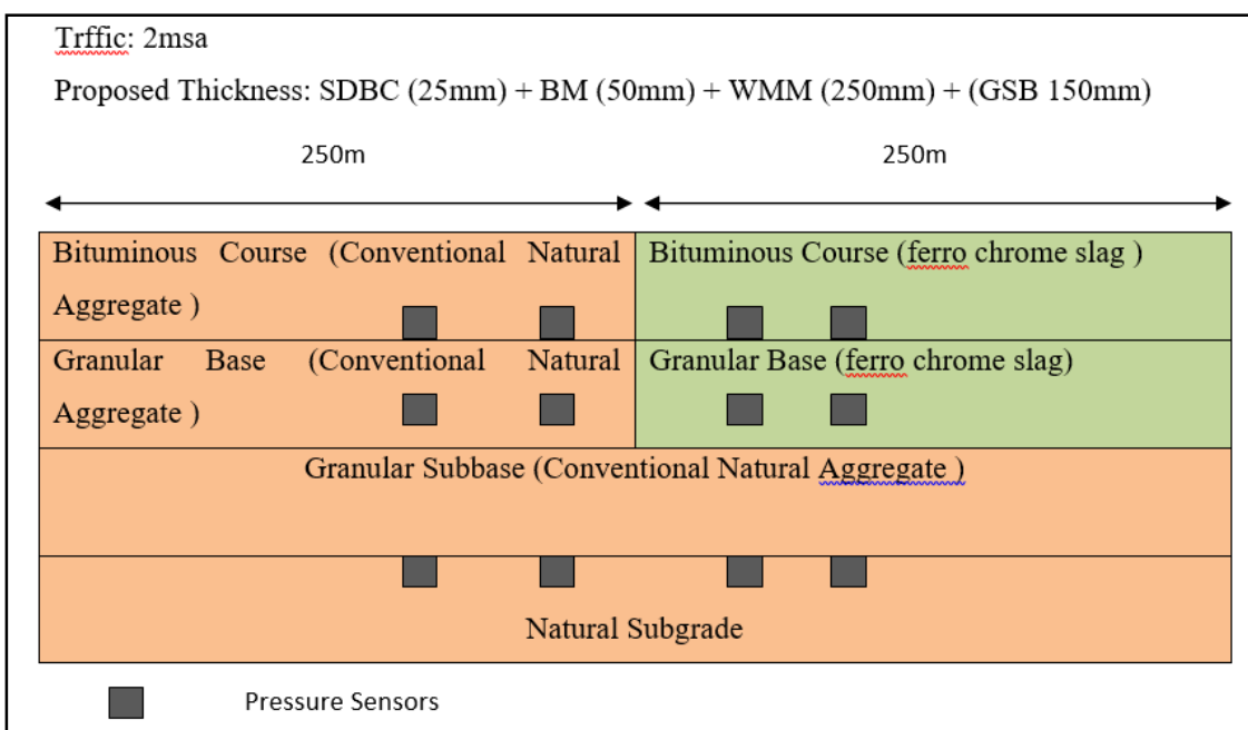
Figure 3: Proposed Layout for Trial Section
